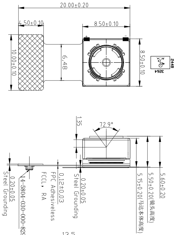
TOP VIEW
